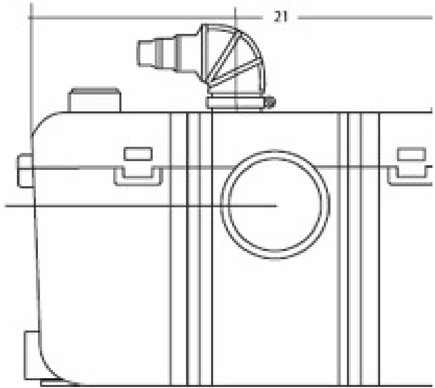
Sanibest macerating unit – dimensions shown in inches
